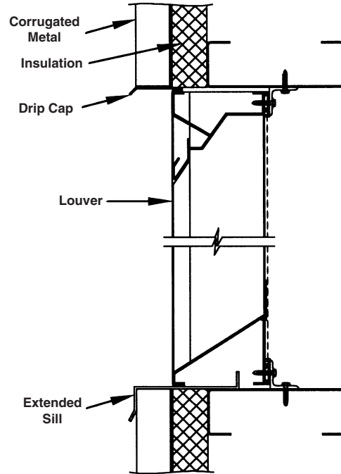
Flange Mount
