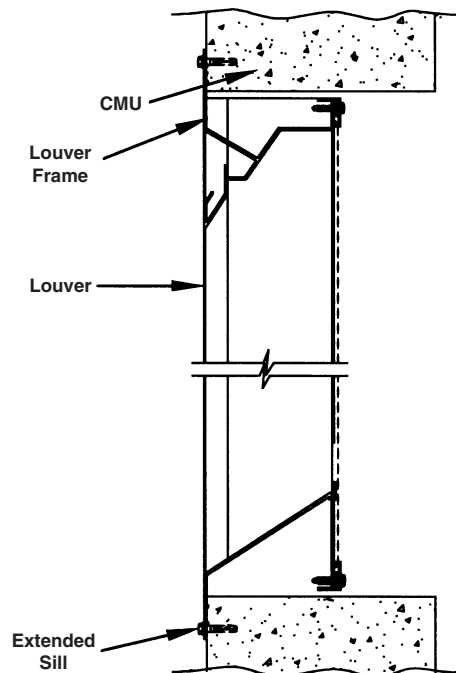
Flange Mount
