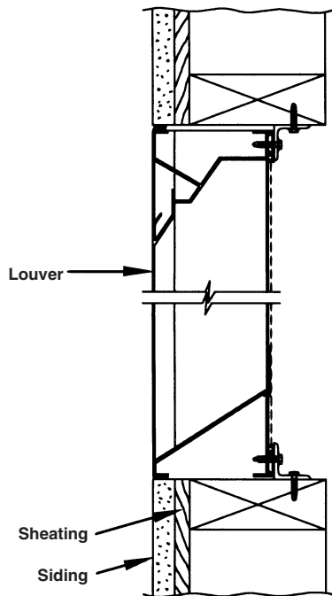
Wood Installation
